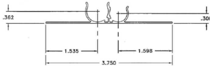
Dimensional Specification (in.)
