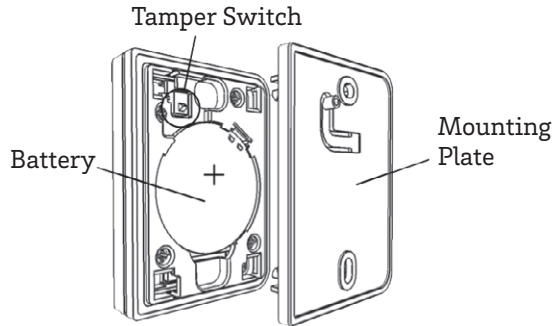
Sensor Back
