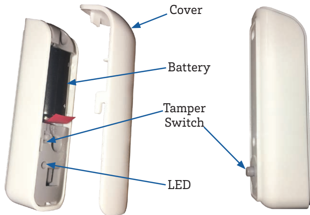
Sensor Front
